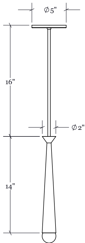
Elevation View Scale 1 : 8
