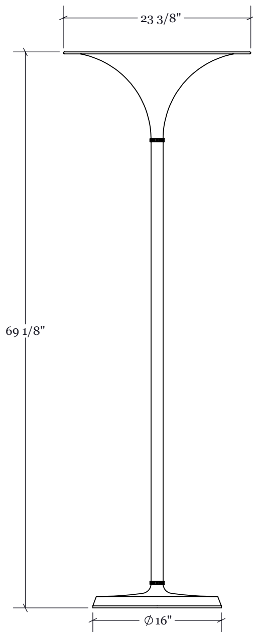
Elevation View Scale 1 : 12
