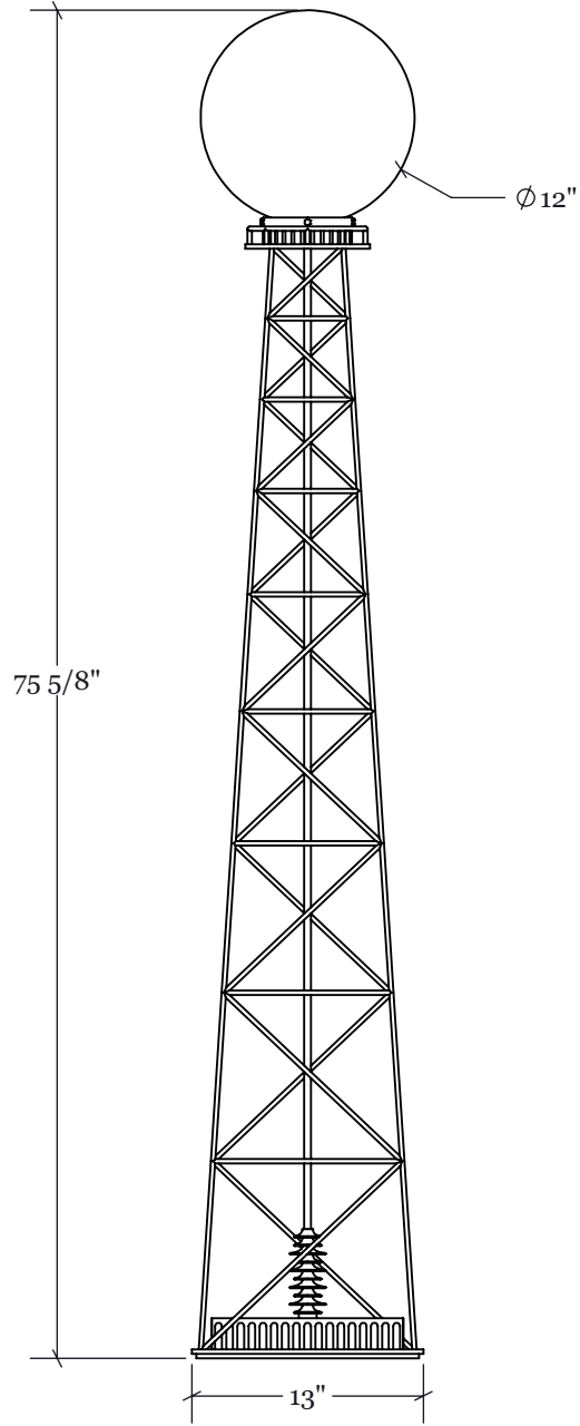
Elevation View Scale 1 : 12
