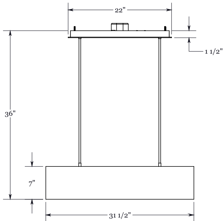
Elevation View Scale 1 : 12
