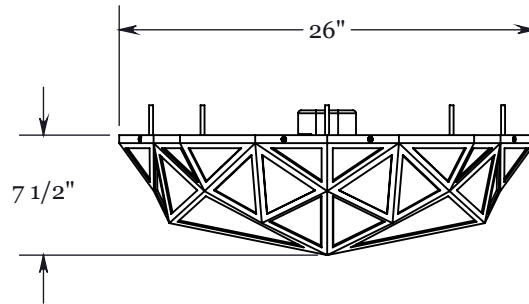
ELEVATION VIEW SCALE 1 : 12
